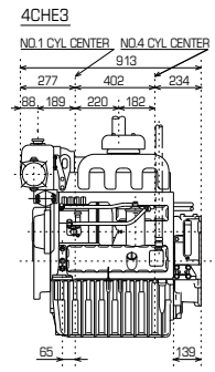
Engine only / Left side view
